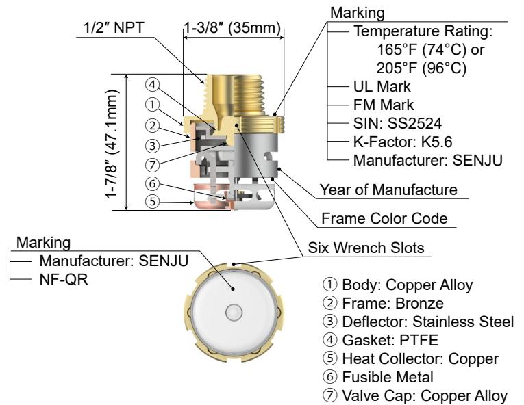
Figure 1: Model NF-QR, K = 5.6 Flush Pendent Sprinkler
